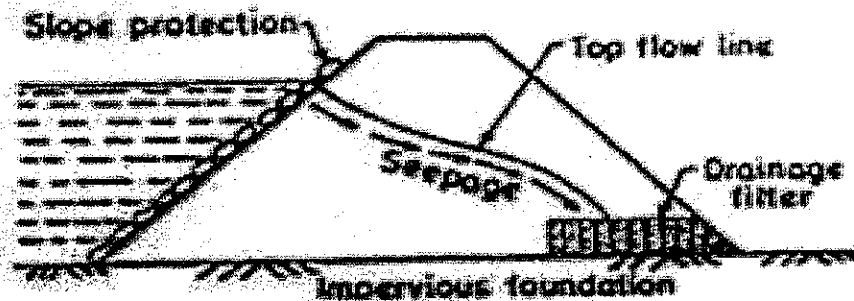
Homogeneous embankment provided with a drainage filter.
