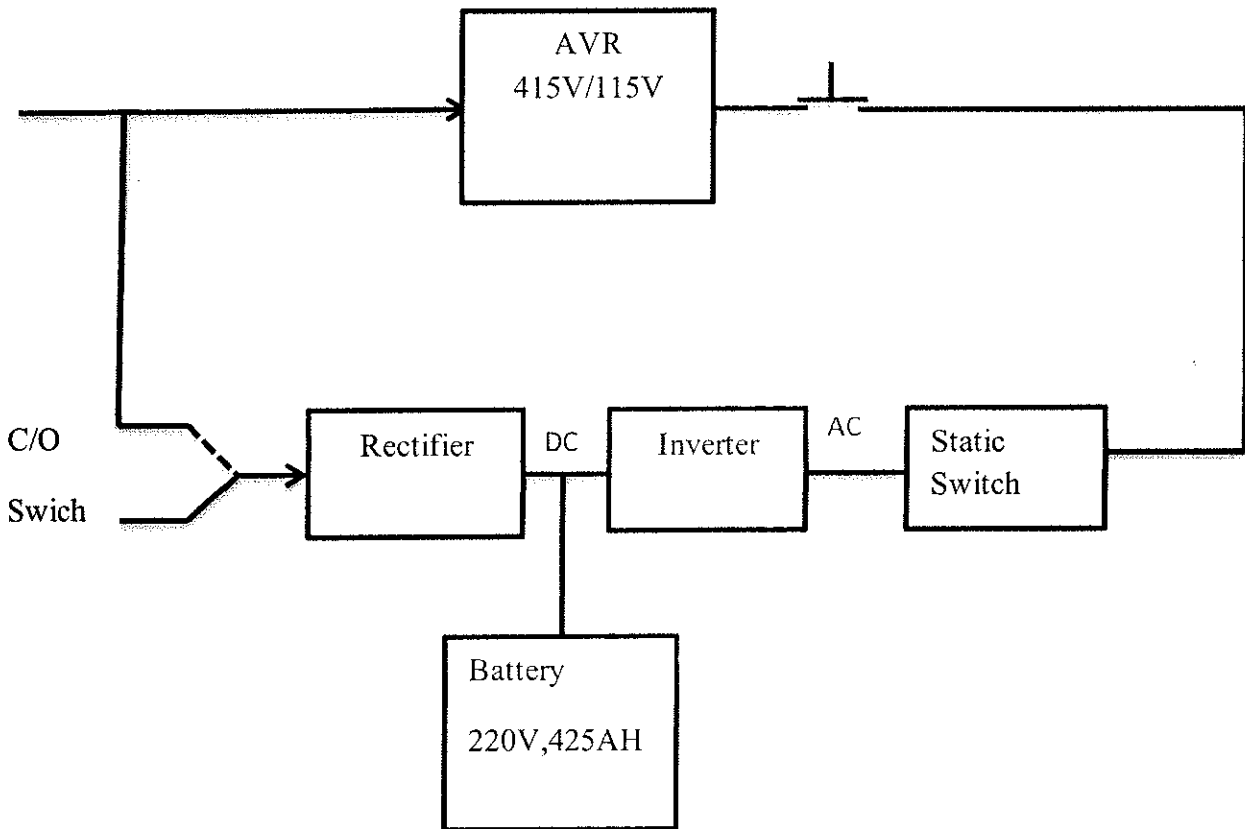
Fig. Block Diagram of UPS
